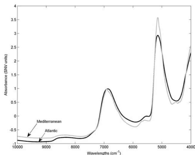
Figure 2. Average NIR spectra of Atlantic (black line) and Mediterranean (gray line) sea salt samples.
